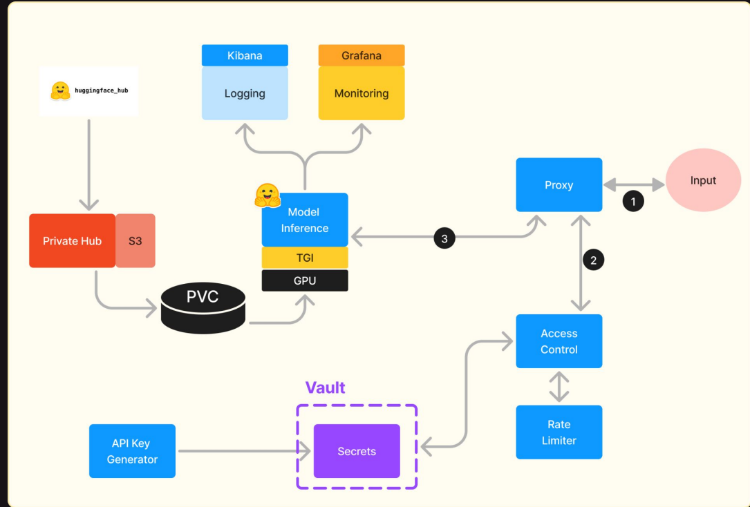
LLM Inference Architecture (Per-model)
