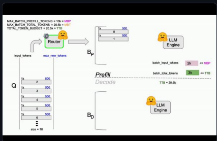
Figure 3: TGI Continuous Batching animation based on TGI router code
