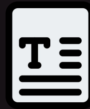
Formatting
