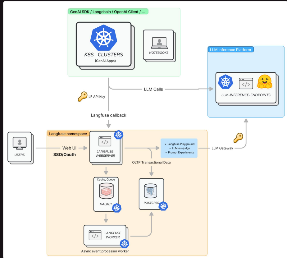
Observability architecture
