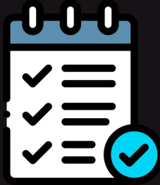
Completeness
