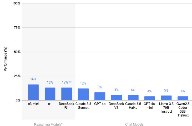
Baseline Hard
